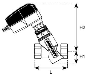
FlowCon GreEQ.0/1 in FlowCon A valve DN15/20/25 (1/2", 3/4", 1") with FlowCon FNR.0.2 actuator
